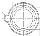
Wormshaft Lock- Slack Adjuster 100813760
