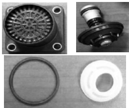
Unloader Plunger Assy with Silencer MSP 3/117
