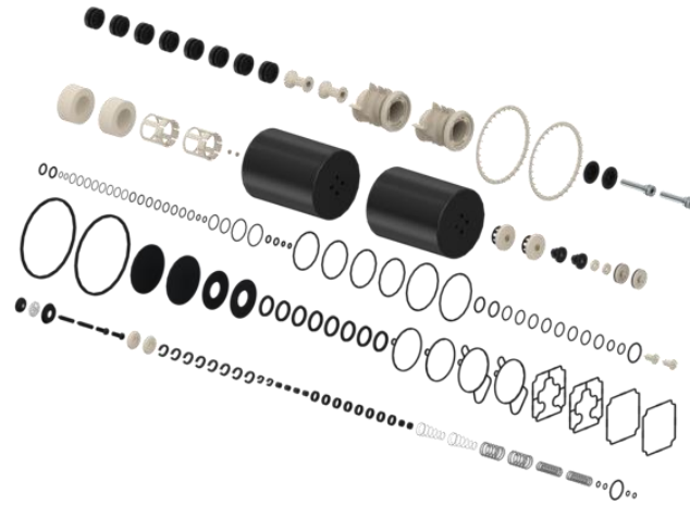
Valve + Silencer 300003128
